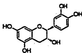
EPICATECHIN
